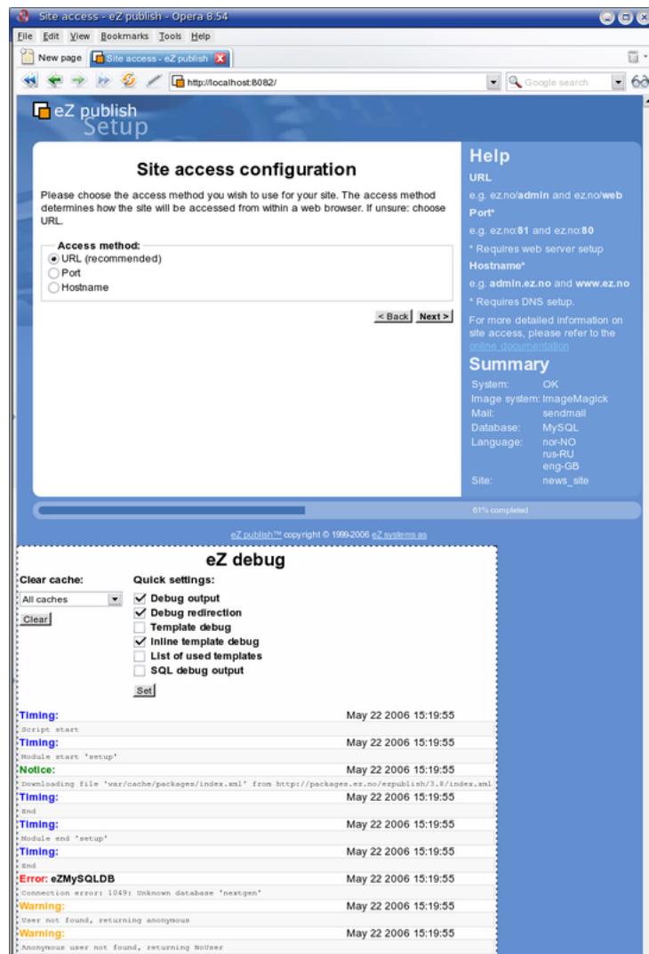
Figure 1.28: The debug output appears at the bottom of the page
