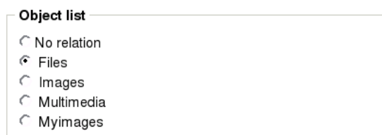
Figure 5.51: Object attribute edit interface for the "Object relations" datatype (list with radio buttons).
